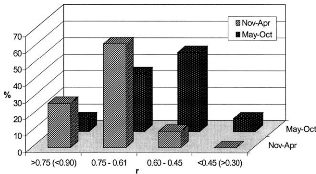
Fig. 3. Ratios of spatial correlations ( r ) of the homogenised PDSI values calculated with the Blaney–Criddle method, May–October, November–April, five settlements, 1901–1990.
