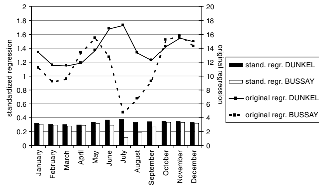
Fig. 2. Original and standardized regression coefficients for the homogenised PDSI values calculated with the Blaney–Criddle method and the soil moisture content time series of Dunkel and Bussay, Szeged.
