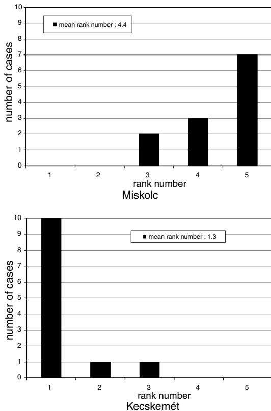
Fig. 1. Distribution of the rank numbers of the standard deviation of the homogenised PDSI data sets, calculated with the Blaney–Criddle method, at Miskolc and Kecskemét. The rank number “1” (“5”) indicates the lowest (highest) standard deviation in the given month.
